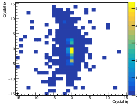
0.1 GeV: Inst. Merged (Circular)
