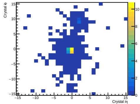
1 GeV: Shower Merging
