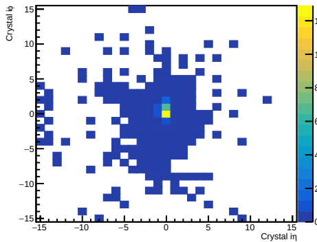
0.5 GeV: Merged (Oval)
